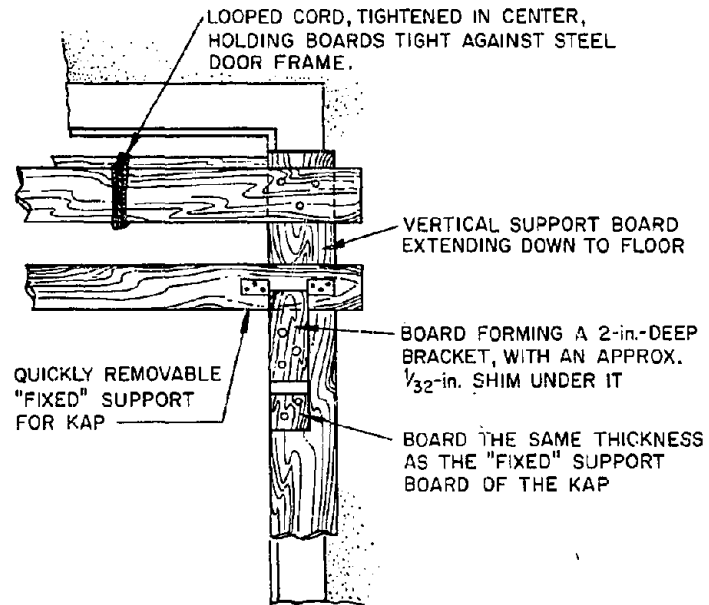
Fig. B-27. Quick-removal bracket for steel-framed doorway.
